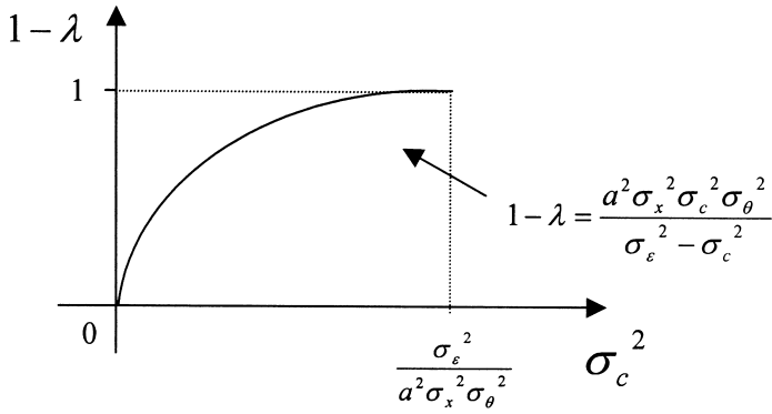
Fig. 2. The relationship between the surviving overconfident traders and overconfidence level.
