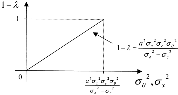
Fig. 1. The relationship between the surviving overconfident traders and either volatility or noise.
